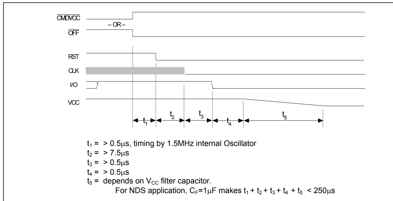
Figure 6: Deactivation Sequence
